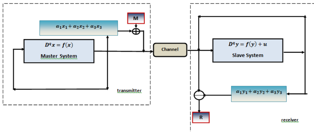
Figure 6: Diagram of secure communication based on anti-synchronization.
