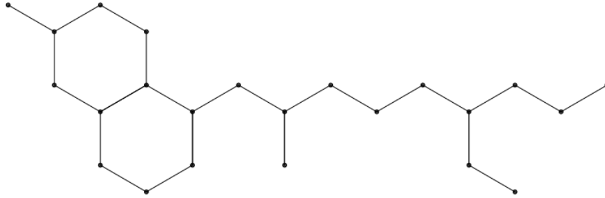
Figure 5- Hydroxychloroquine 2D molecular graph.
