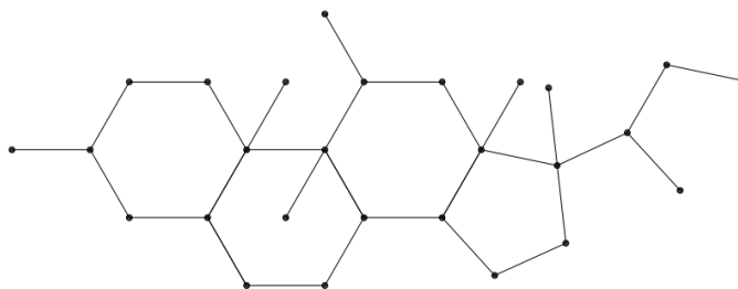
Figure 1- Dexamethasone 2D molecular graph.
