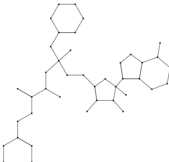
Figure 7- Remdesivir molecular graph.
